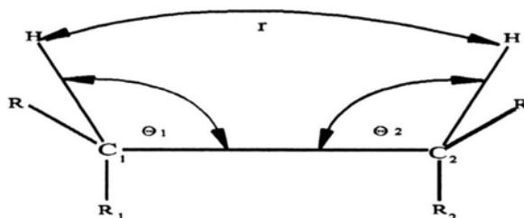
Fig. 2. Schematic representation of the ethane fragment. C_1 and C_2 denote the carbon atoms directed towards the coupled hydrogen atoms H. The internal bond angles H-C 1 -C 2 and H-C 2 -C 1 are denoted by \theta_1 and \theta_2 , respectively. The intramolecular distance between coupling protons is denoted by r . Rs denote part of ring, whereas R_1 and R_2 are substituents.
